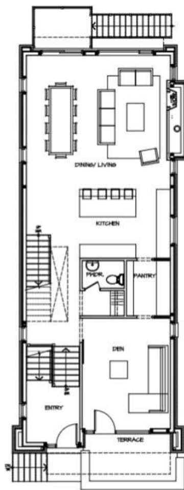
304 Selby Avenue Floor Plan
